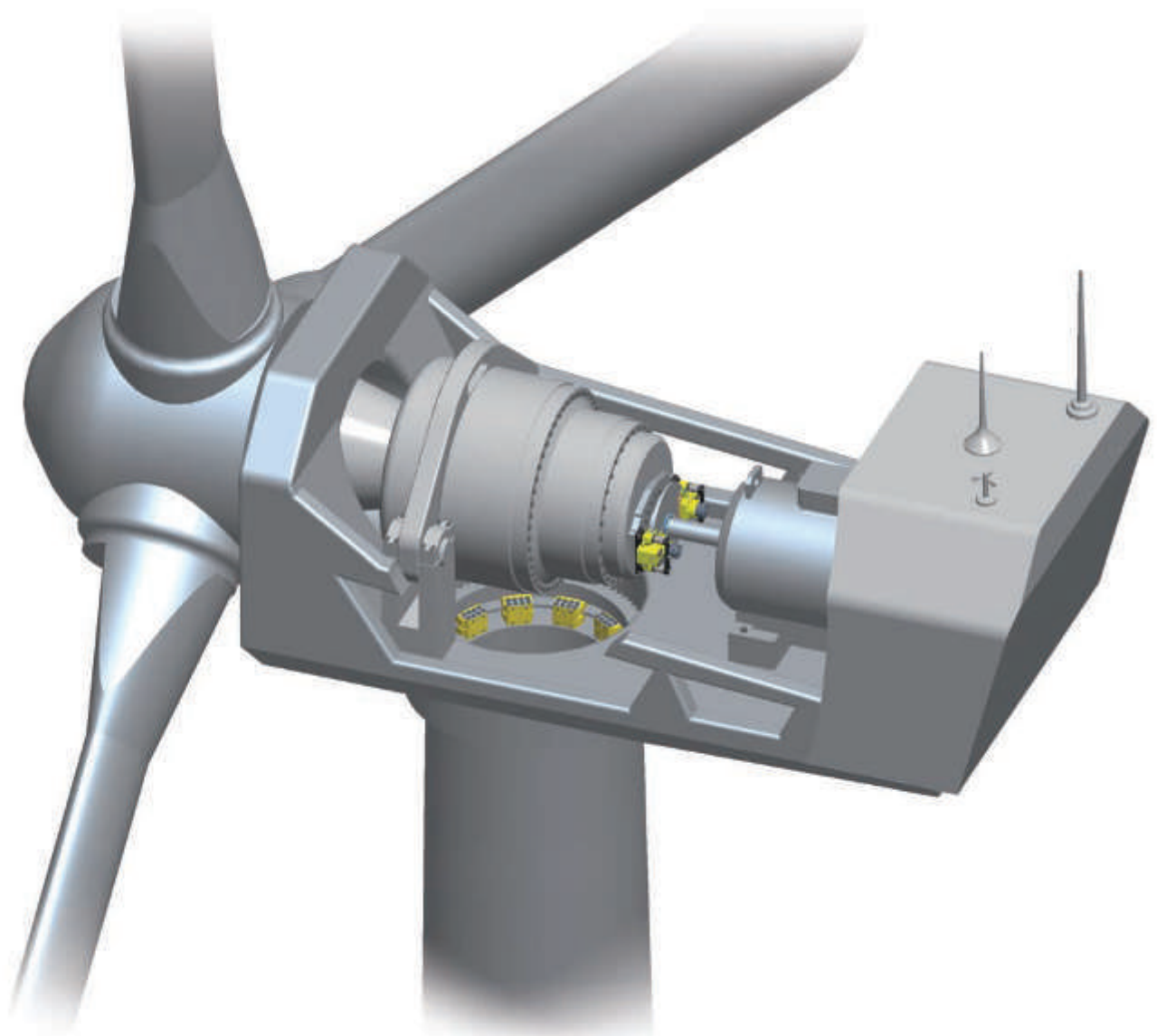
Wind turbines
