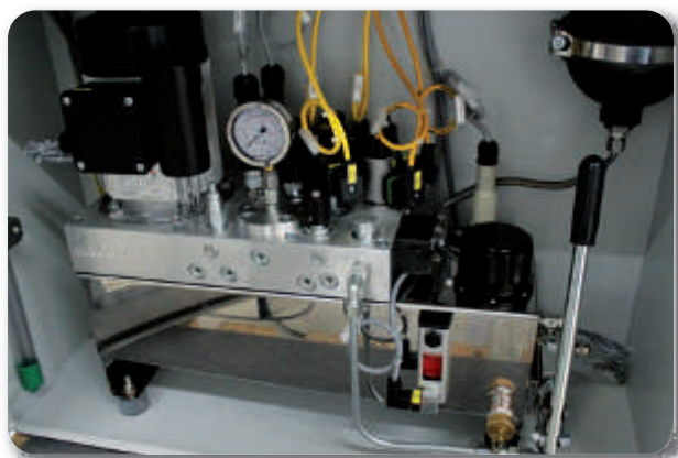
Hydraulic powerpack
