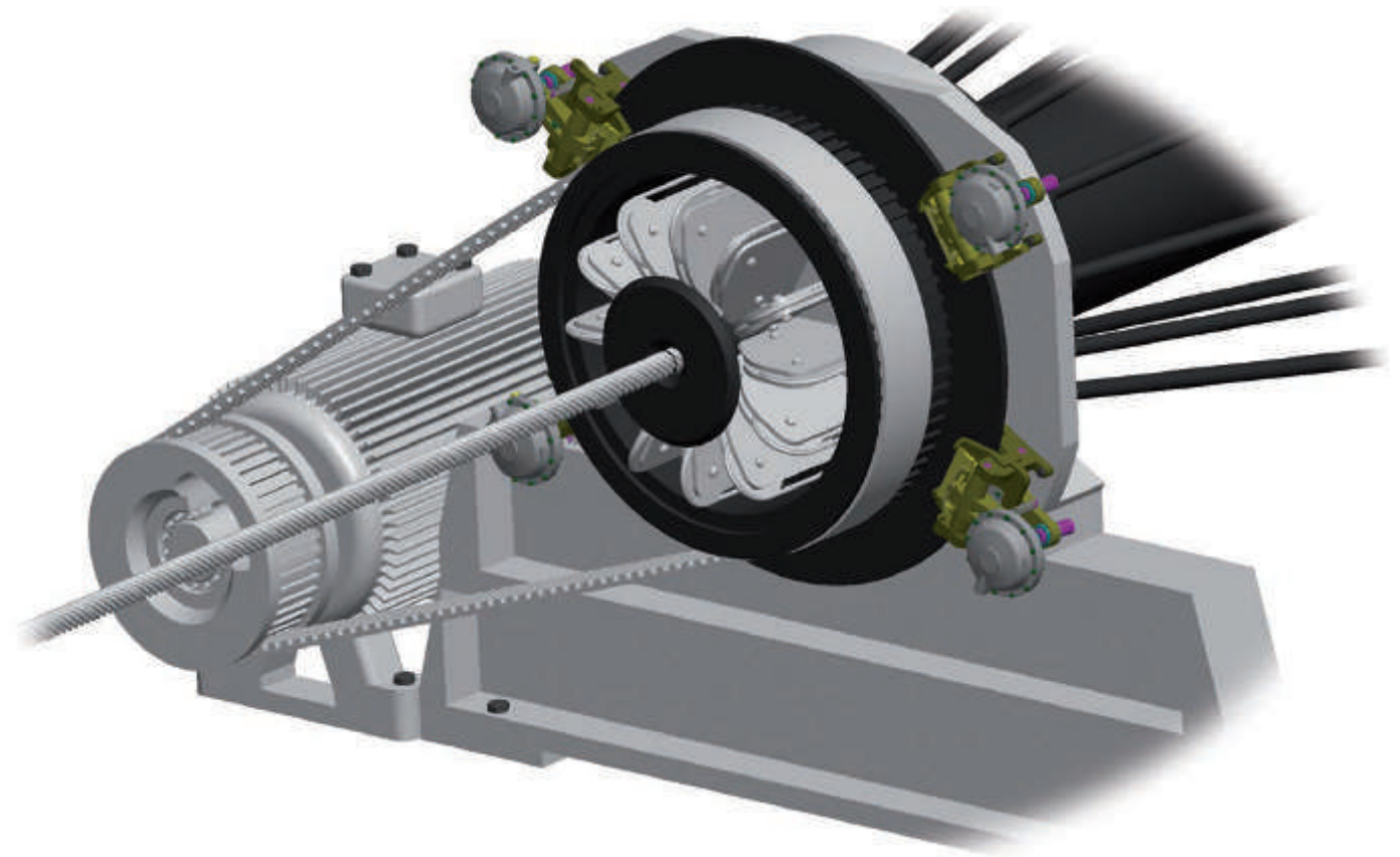
Stranding lines
